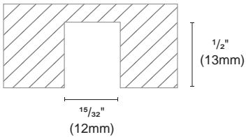
△ Cut out : 15/32"X1/2" (12X13mm)
